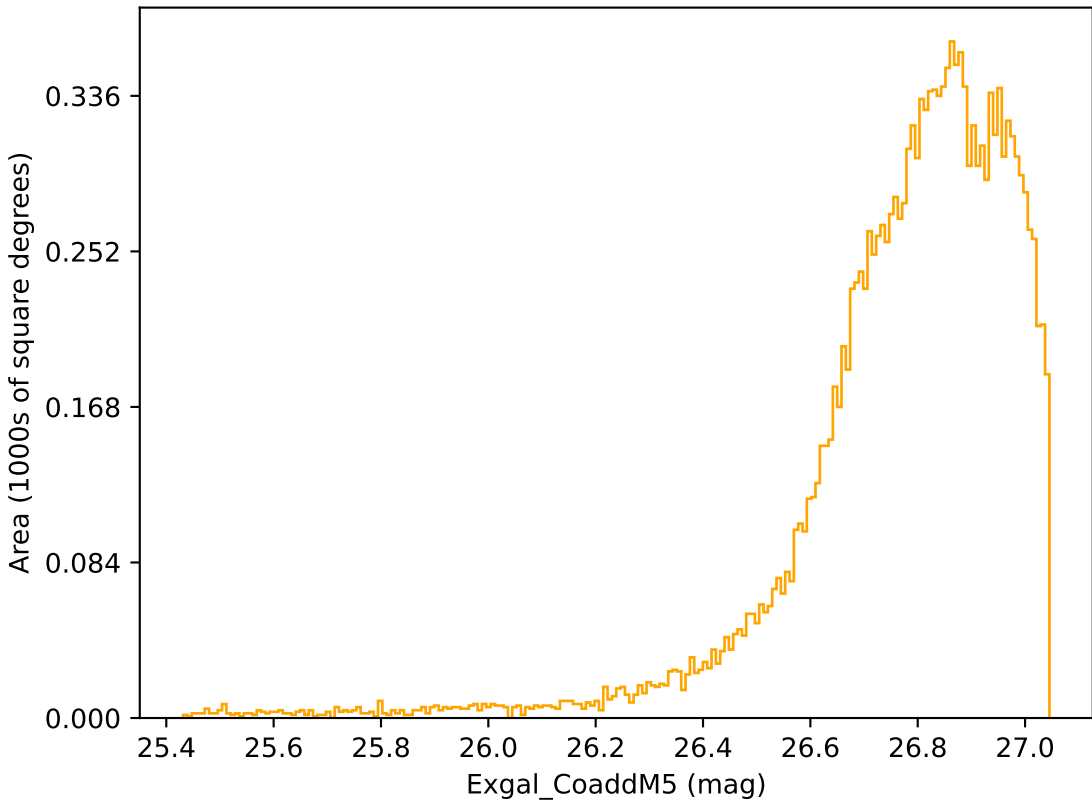
weather_cloudso31v3.4_10yrs WFD r band: Exgal_CoaddM5
