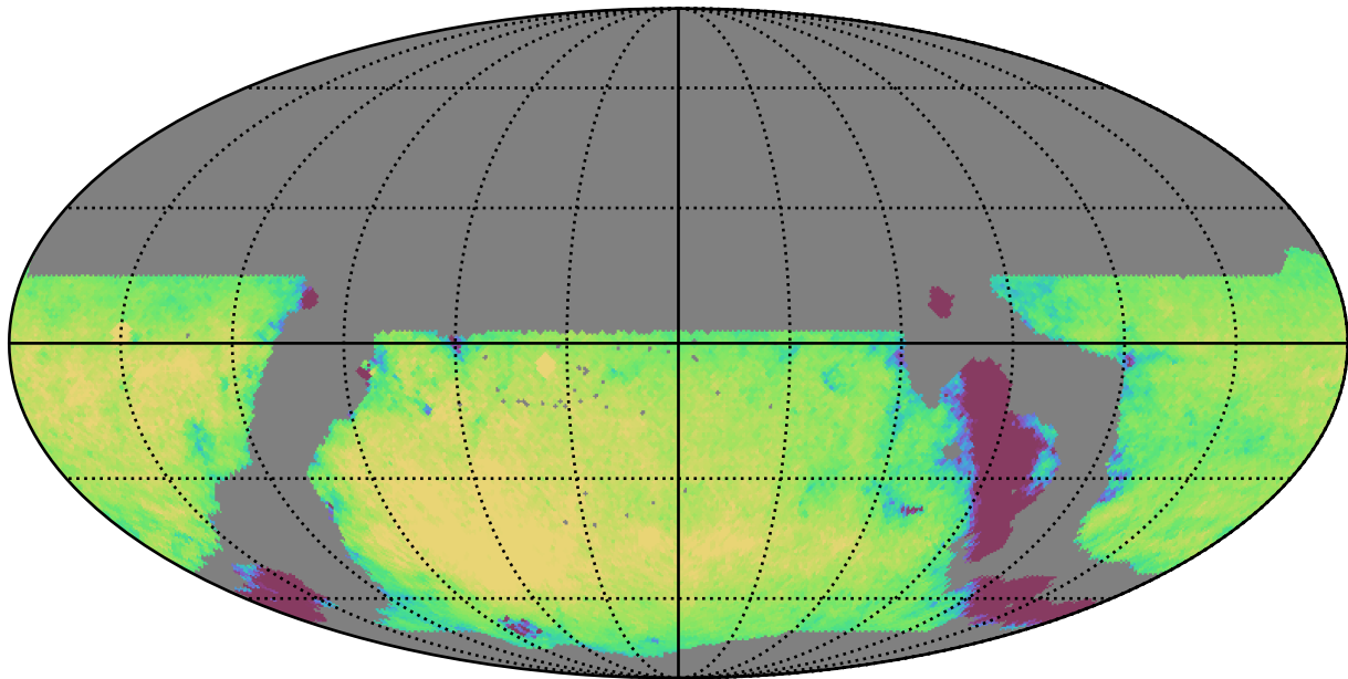
weather_cloudso31v3.4_10yrs WFD g band: Exgal_CoaddM5
