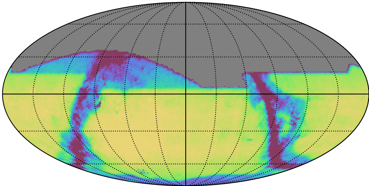
weather_cloudso31v3.4_10yrs All sky z band: Exgal_CoaddM5
