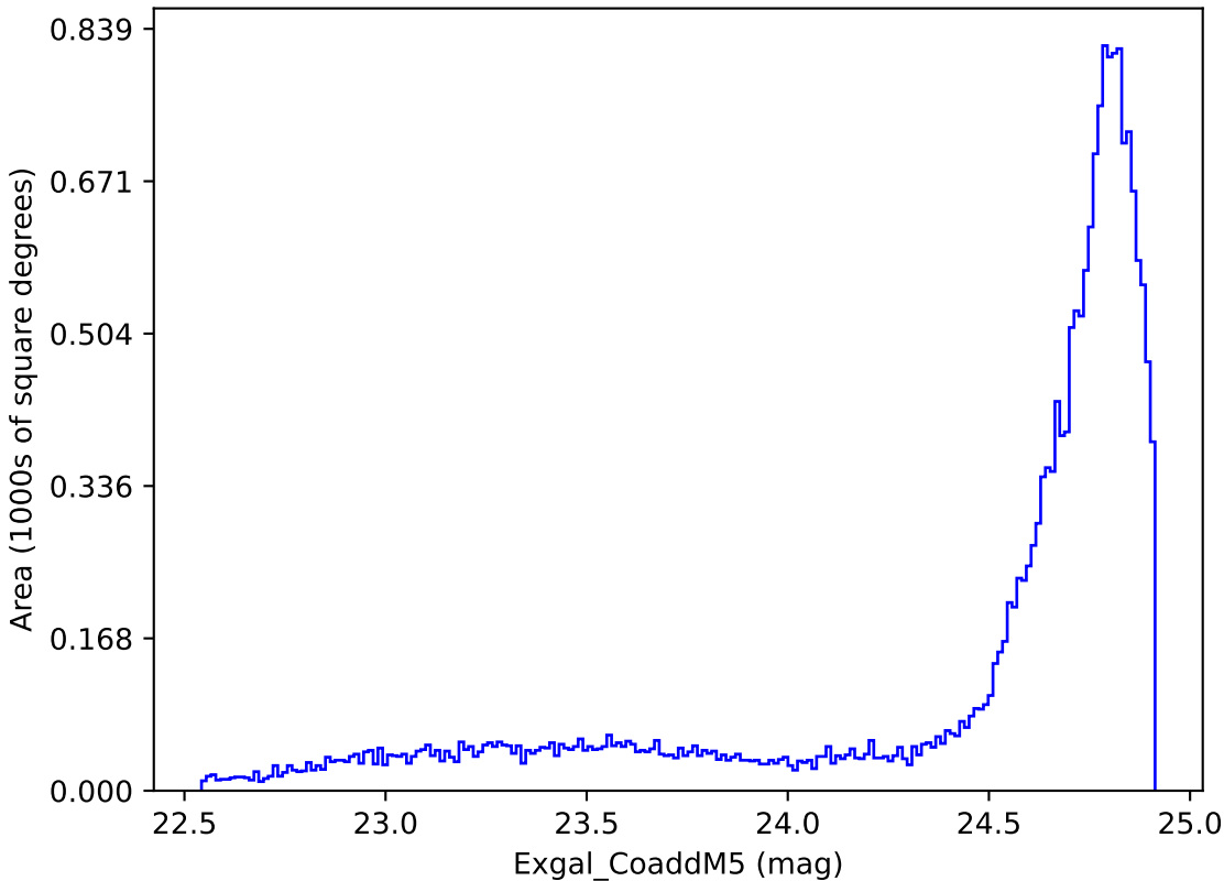
weather_cloudso31v3.4_10yrs All sky y band: Exgal_CoaddM5
