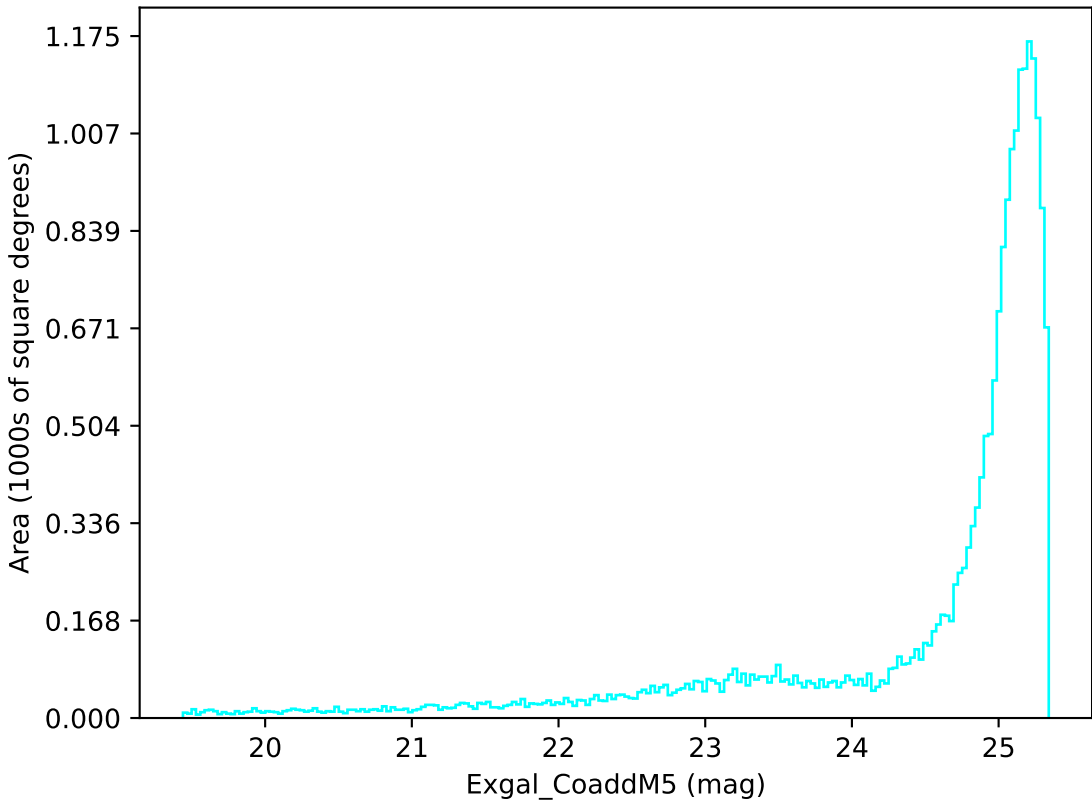
weather_cloudso31v3.4_10yrs All sky u band: Exgal_CoaddM5
