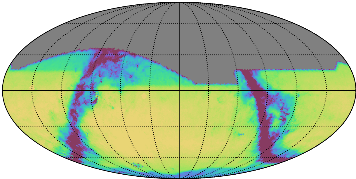
weather_cloudso31v3.4_10yrs All sky r band: Exgal_CoaddM5
