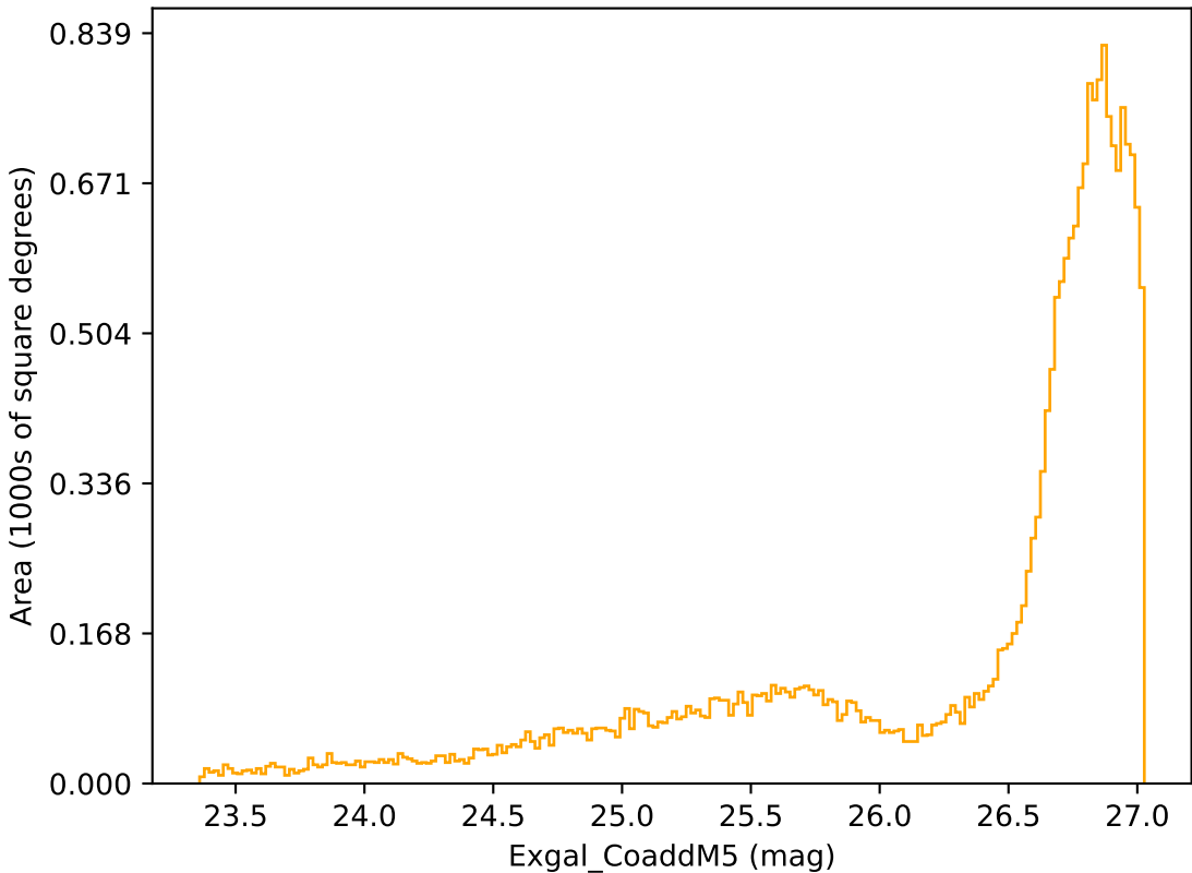
weather_cloudso31v3.4_10yrs All sky r band: Exgal_CoaddM5
