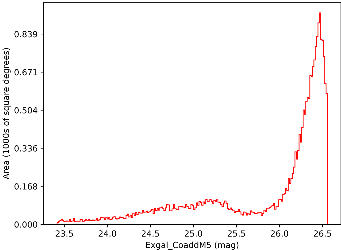
weather_cloudso31v3.4_10yrs All sky i band: Exgal_CoaddM5
