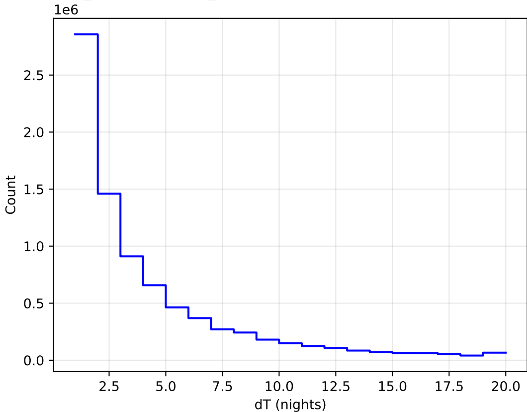
weather_cloudso31v3.4_10yrs WFD all bands: DeltaNight Histogram
