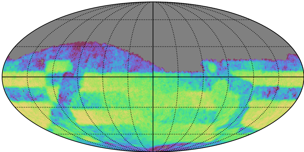
weather_cloudso31v3.4_10yrs Yr 3-4 z band: CoaddM5
