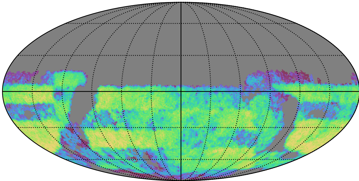
weather_cloudso31v3.4_10yrs Yr 3-4 u band: CoaddM5
