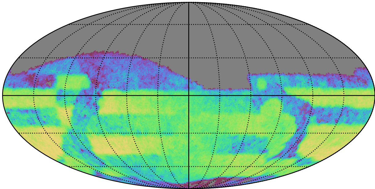
weather_cloudso31v3.4_10yrs Yr 3-4 r band: CoaddM5
