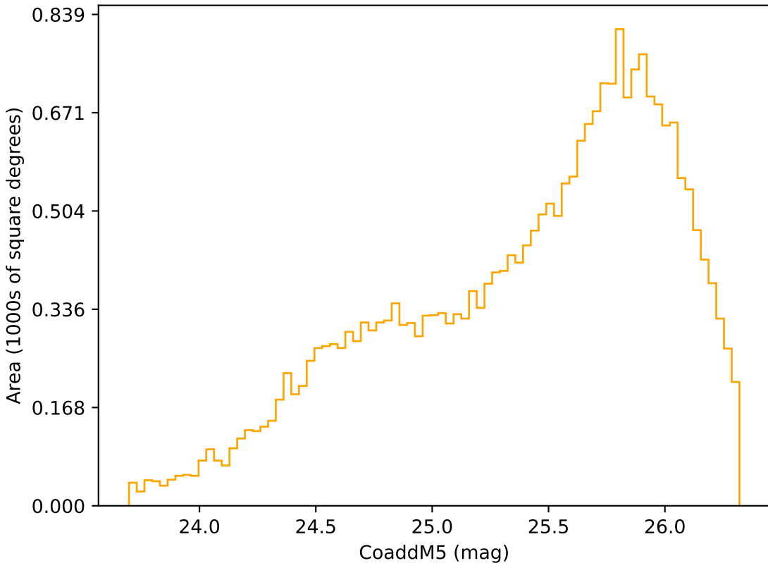
weather_cloudso31v3.4_10yrs Yr 3-4 r band: CoaddM5
