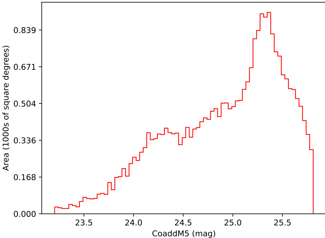
weather_cloudso31v3.4_10yrs Yr 3-4 i band: CoaddM5
