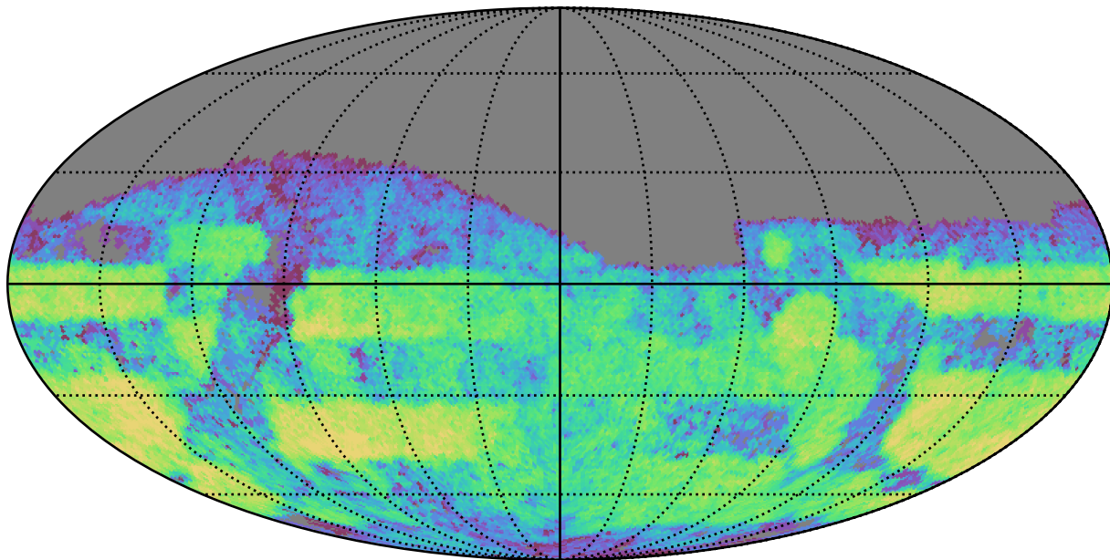
weather_cloudso31v3.4_10yrs Yr 3-4 g band: CoaddM5
