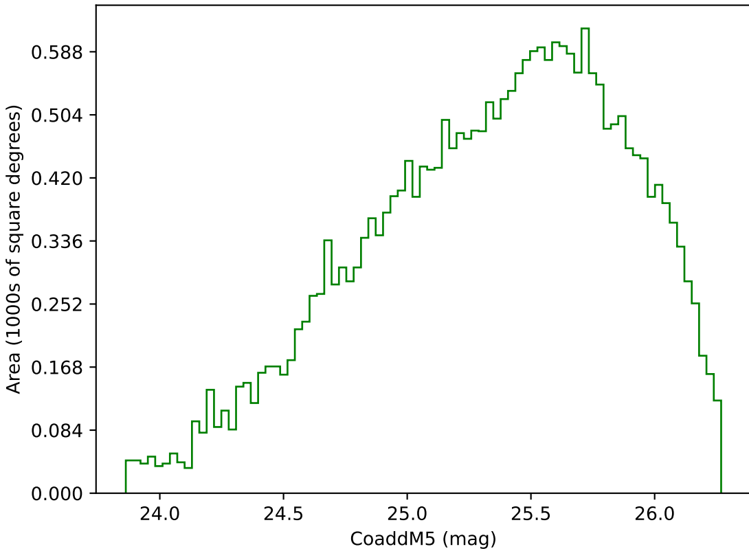
weather_cloudso31v3.4_10yrs Yr 3-4 g band: CoaddM5
