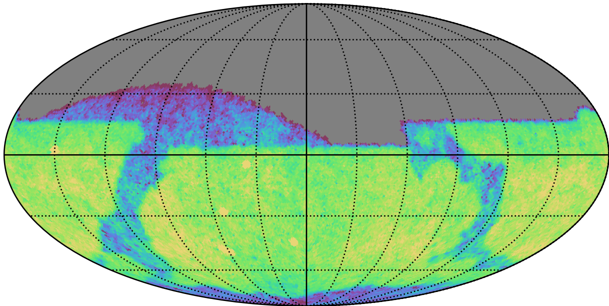
weather_cloudso31v3.4_10yrs Yr 1 z band: CoaddM5
