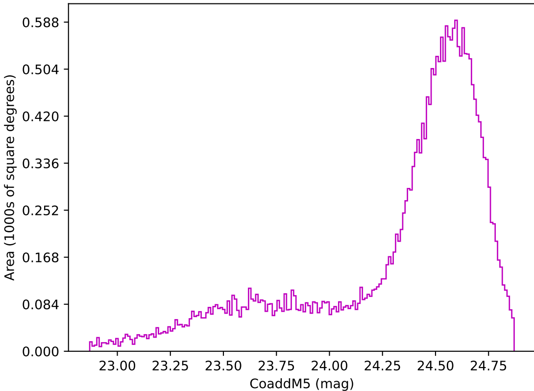
weather_cloudso31v3.4_10yrs Yr 1 z band: CoaddM5
