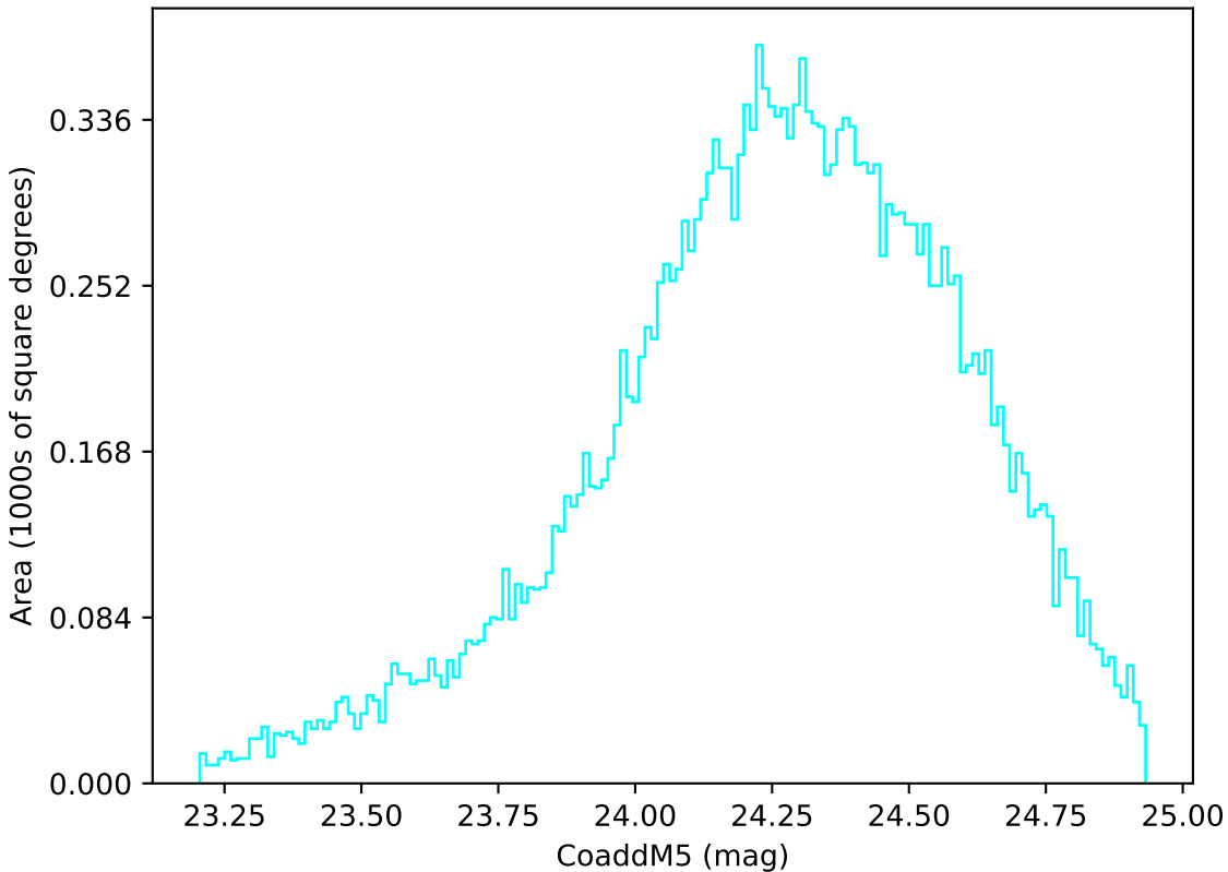
weather_cloudso31v3.4_10yrs Yr 1 u band: CoaddM5
