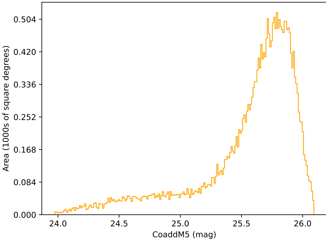
weather_cloudso31v3.4_10yrs Yr 1 r band: CoaddM5
