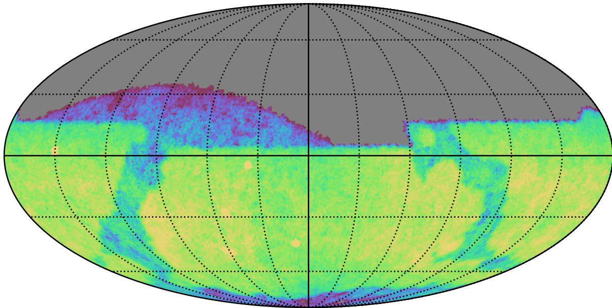
weather_cloudso31v3.4_10yrs Yr 1 i band: CoaddM5
