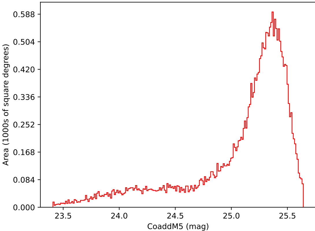
weather_cloudso31v3.4_10yrs Yr 1 i band: CoaddM5
