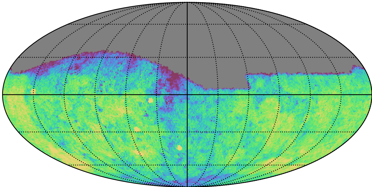
weather_cloudso31v3.4_10yrs Yr 1 g band: CoaddM5
