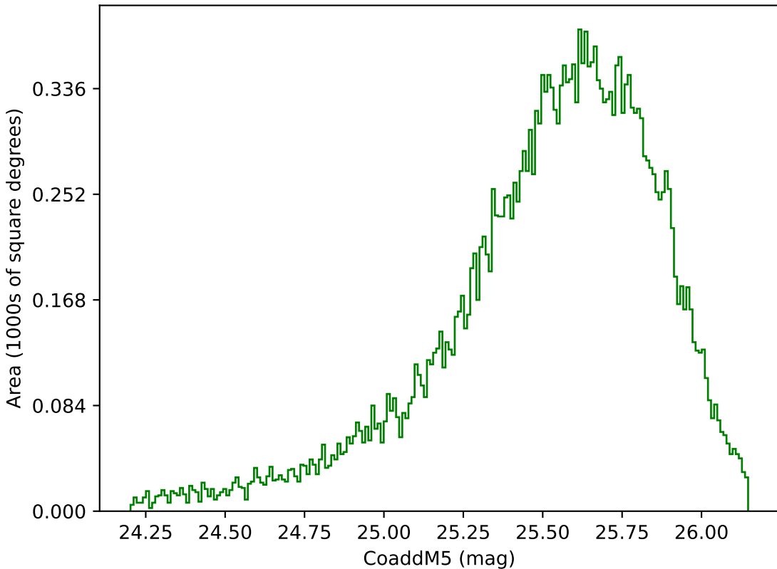
weather_cloudso31v3.4_10yrs Yr 1 g band: CoaddM5
