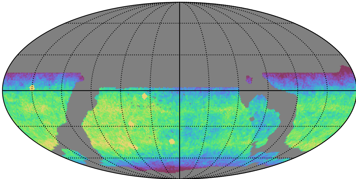
weather_cloudso31v3.4_10yrs WFD z band: CoaddM5
