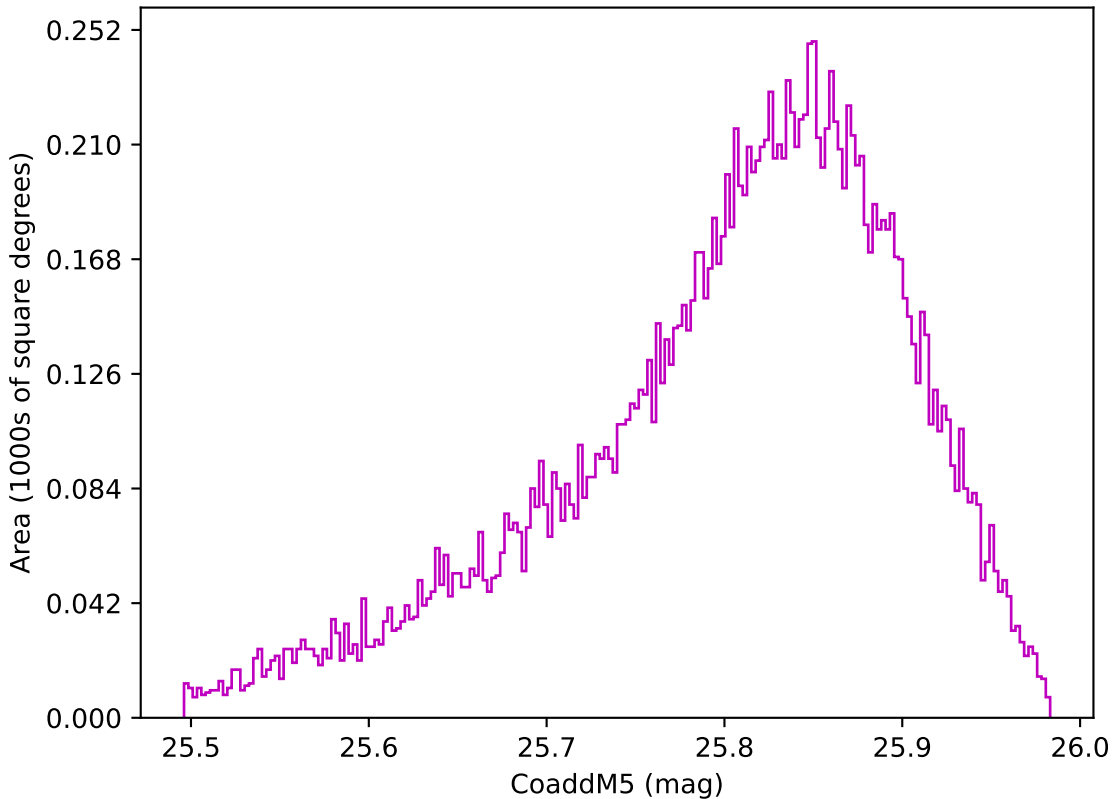
weather_cloudso31v3.4_10yrs WFD z band: CoaddM5
