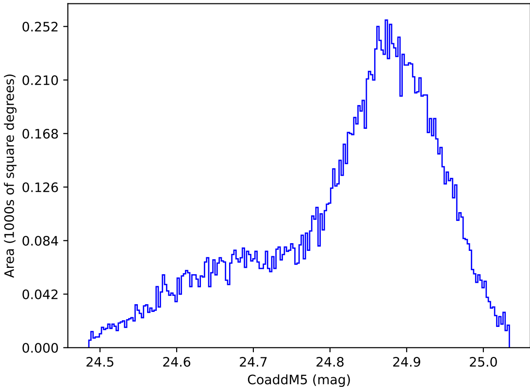
weather_cloudso31v3.4_10yrs WFD y band: CoaddM5
