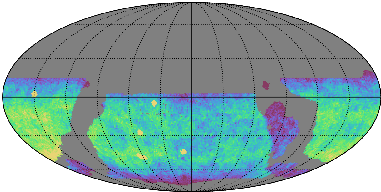
weather_cloudso31v3.4_10yrs WFD u band: CoaddM5
