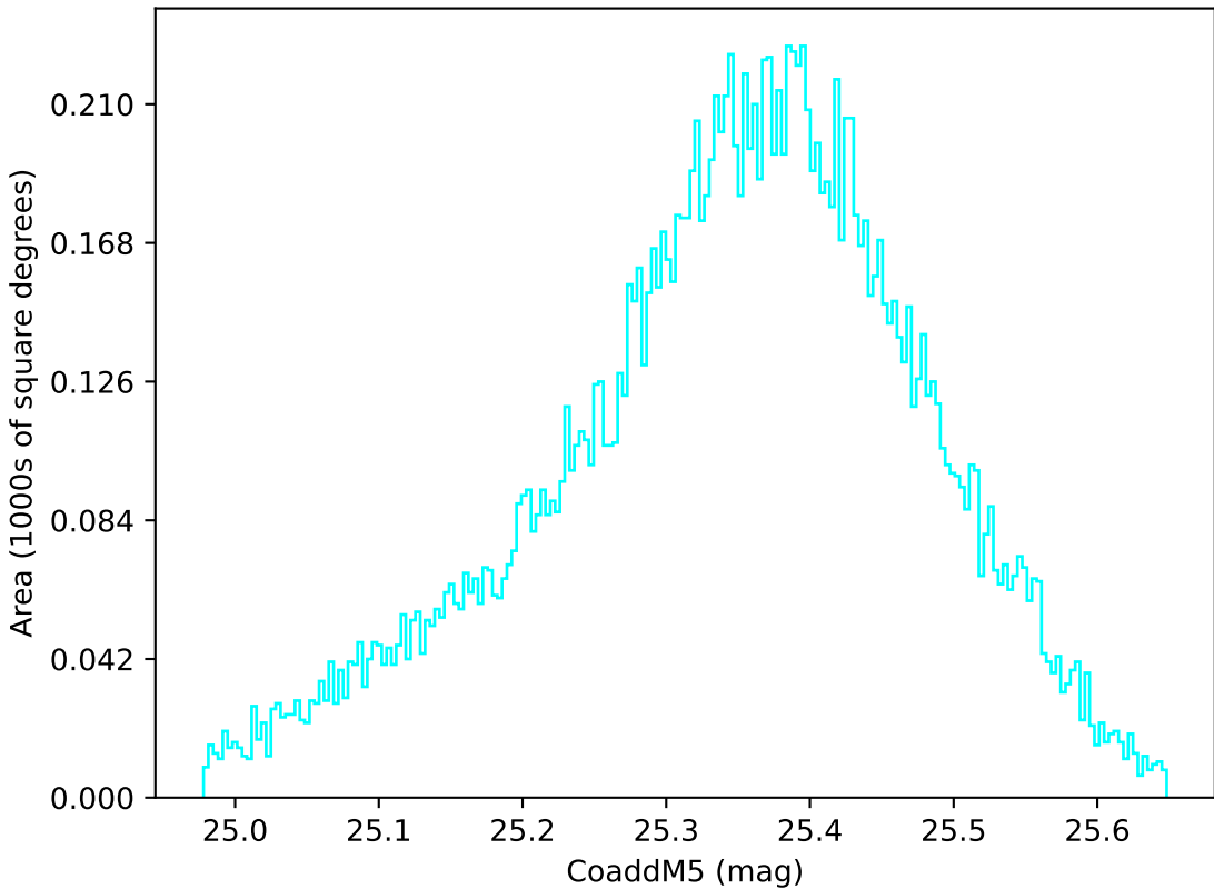
weather_cloudso31v3.4_10yrs WFD u band: CoaddM5
