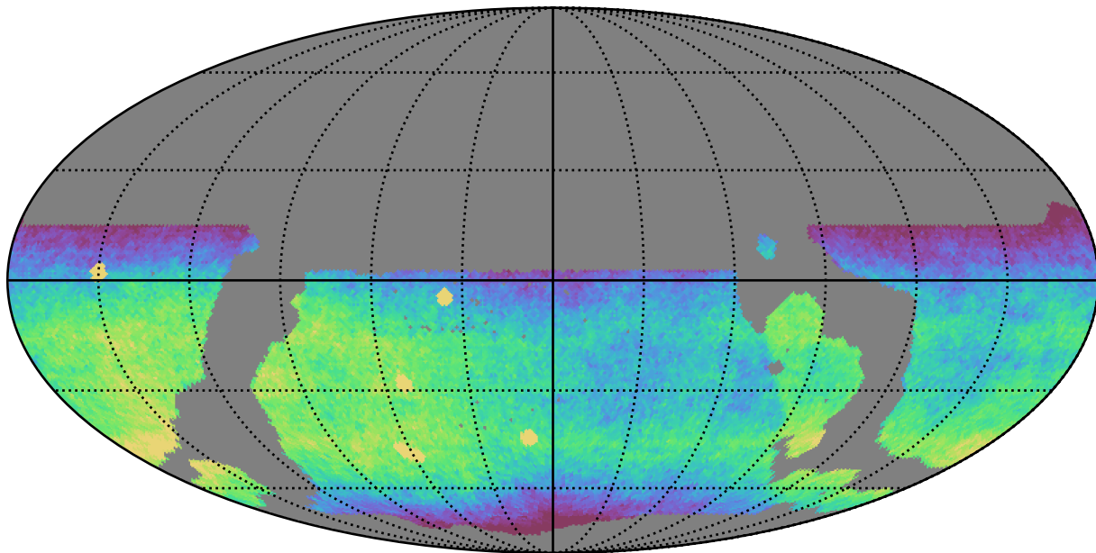
weather_cloudso31v3.4_10yrs WFD r band: CoaddM5
