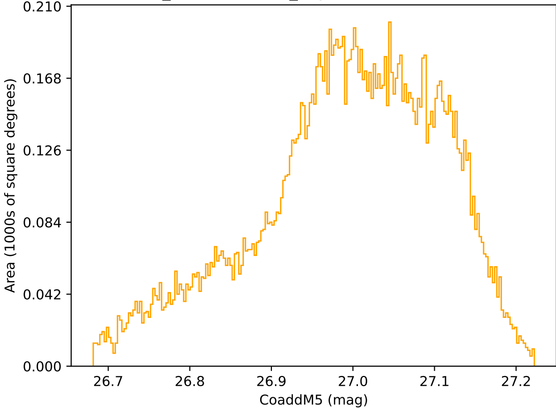
weather_cloudso31v3.4_10yrs WFD r band: CoaddM5
