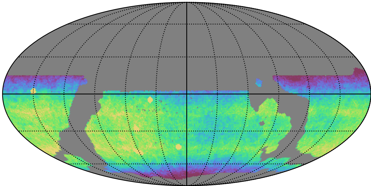
weather_cloudso31v3.4_10yrs WFD i band: CoaddM5
