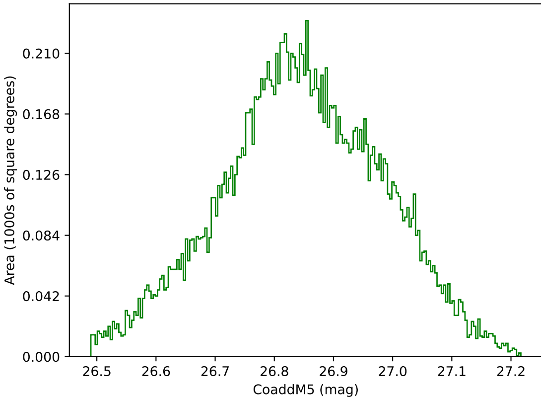
weather_cloudso31v3.4_10yrs WFD g band: CoaddM5
