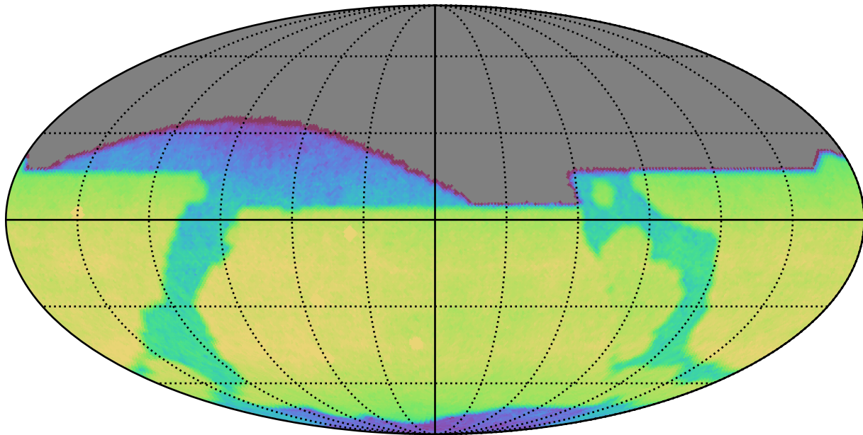
weather_cloudso31v3.4_10yrs All sky z band: CoaddM5
