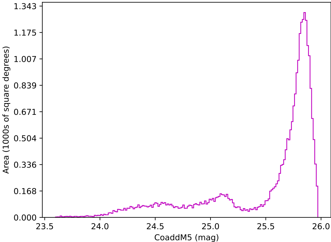
weather_cloudso31v3.4_10yrs All sky z band: CoaddM5
