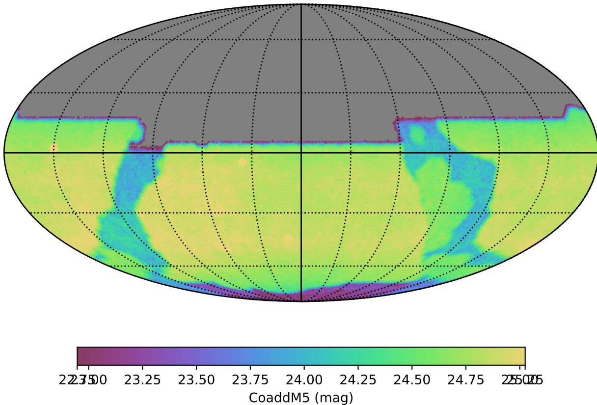
weather_cloudso31v3.4_10yrs All sky y band: CoaddM5
