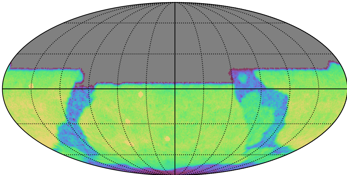
weather_cloudso31v3.4_10yrs All sky u band: CoaddM5
