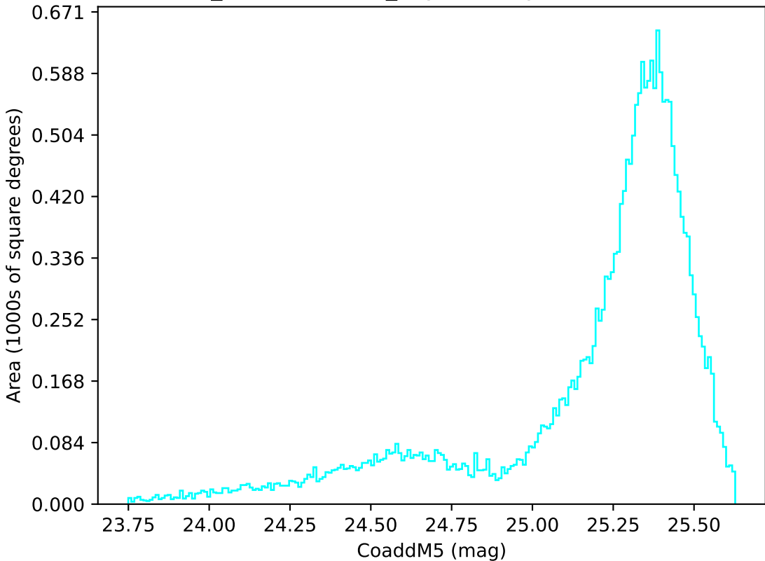
weather_cloudso31v3.4_10yrs All sky u band: CoaddM5
