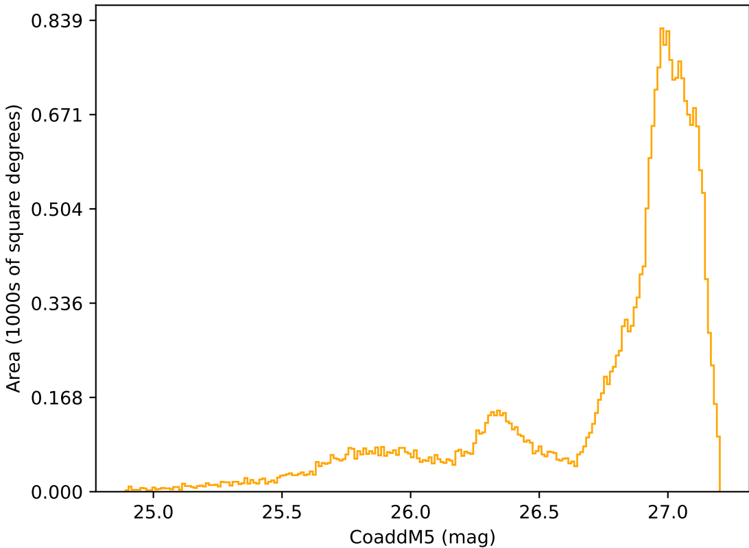
weather_cloudso31v3.4_10yrs All sky r band: CoaddM5
