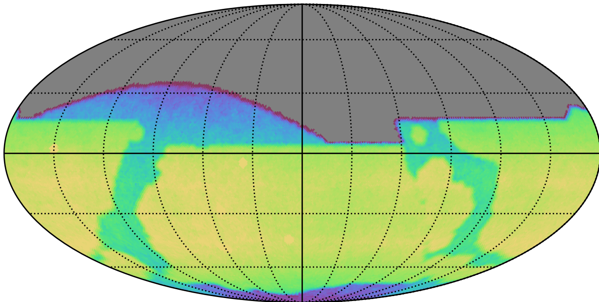
weather_cloudso31v3.4_10yrs All sky i band: CoaddM5
