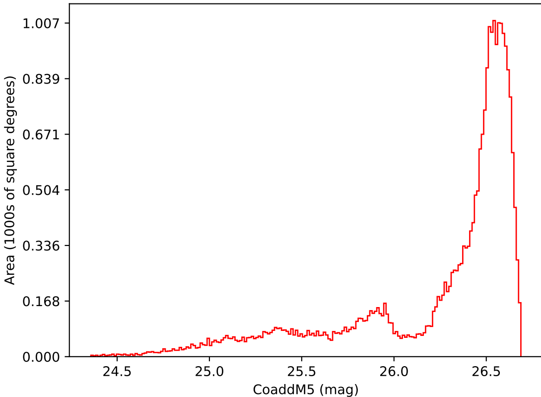
weather_cloudso31v3.4_10yrs All sky i band: CoaddM5
