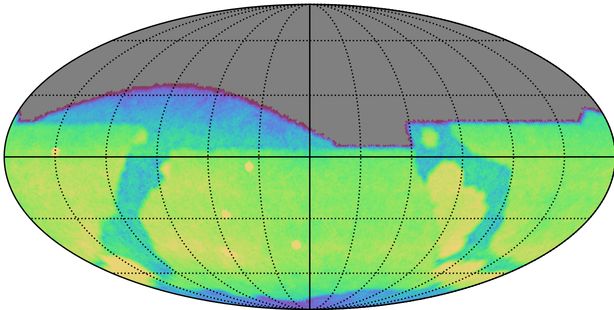
weather_cloudso31v3.4_10yrs All sky g band: CoaddM5
