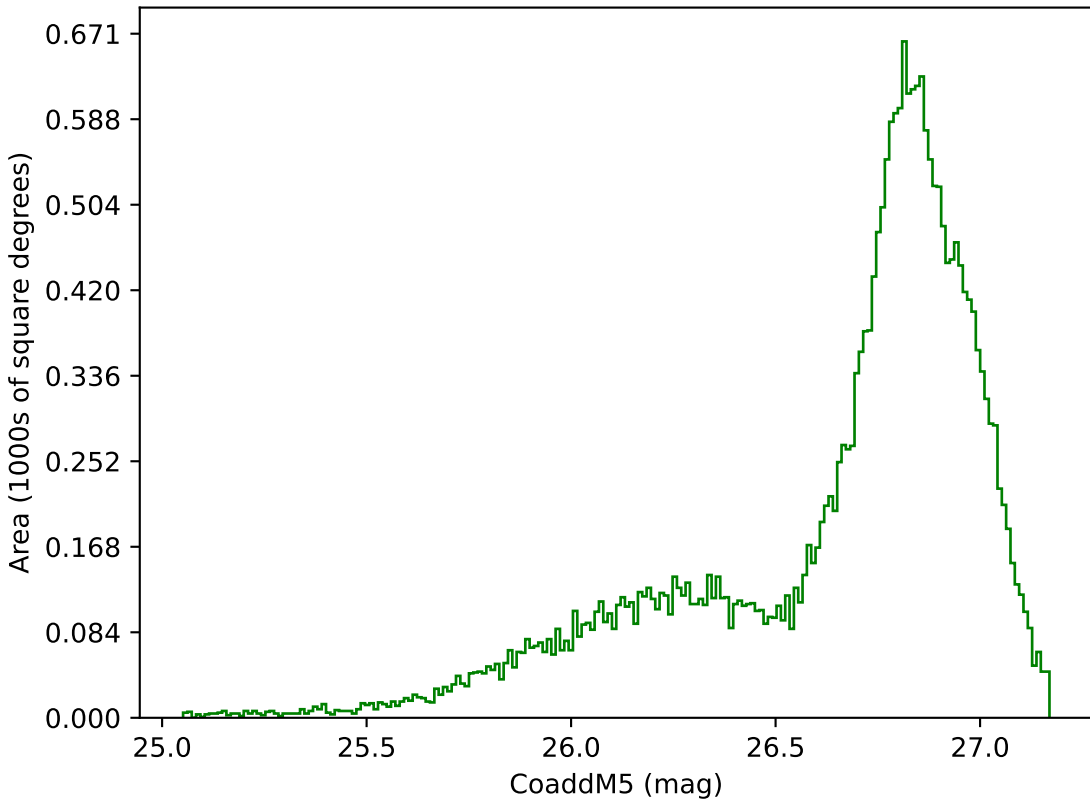
weather_cloudso31v3.4_10yrs All sky g band: CoaddM5
