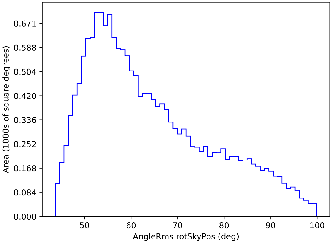
weather_cloudso31v3.4_10yrs WFD u band: AngleRms rotSkyPos
