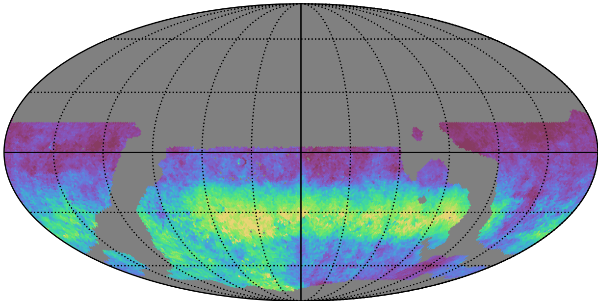
weather_cloudso31v3.4_10yrs WFD g band: AngleRms rotSkyPos
