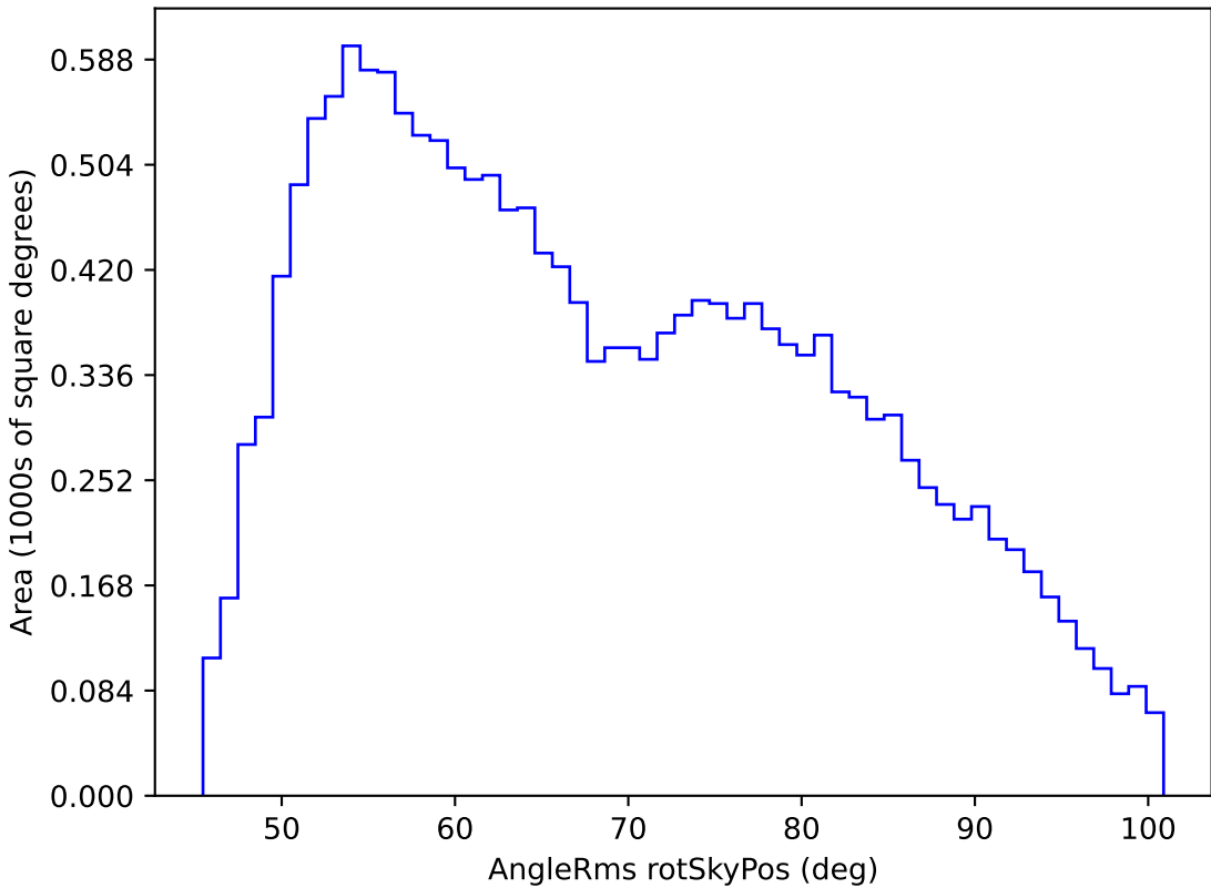
weather_cloudso31v3.4_10yrs WFD g band: AngleRms rotSkyPos
