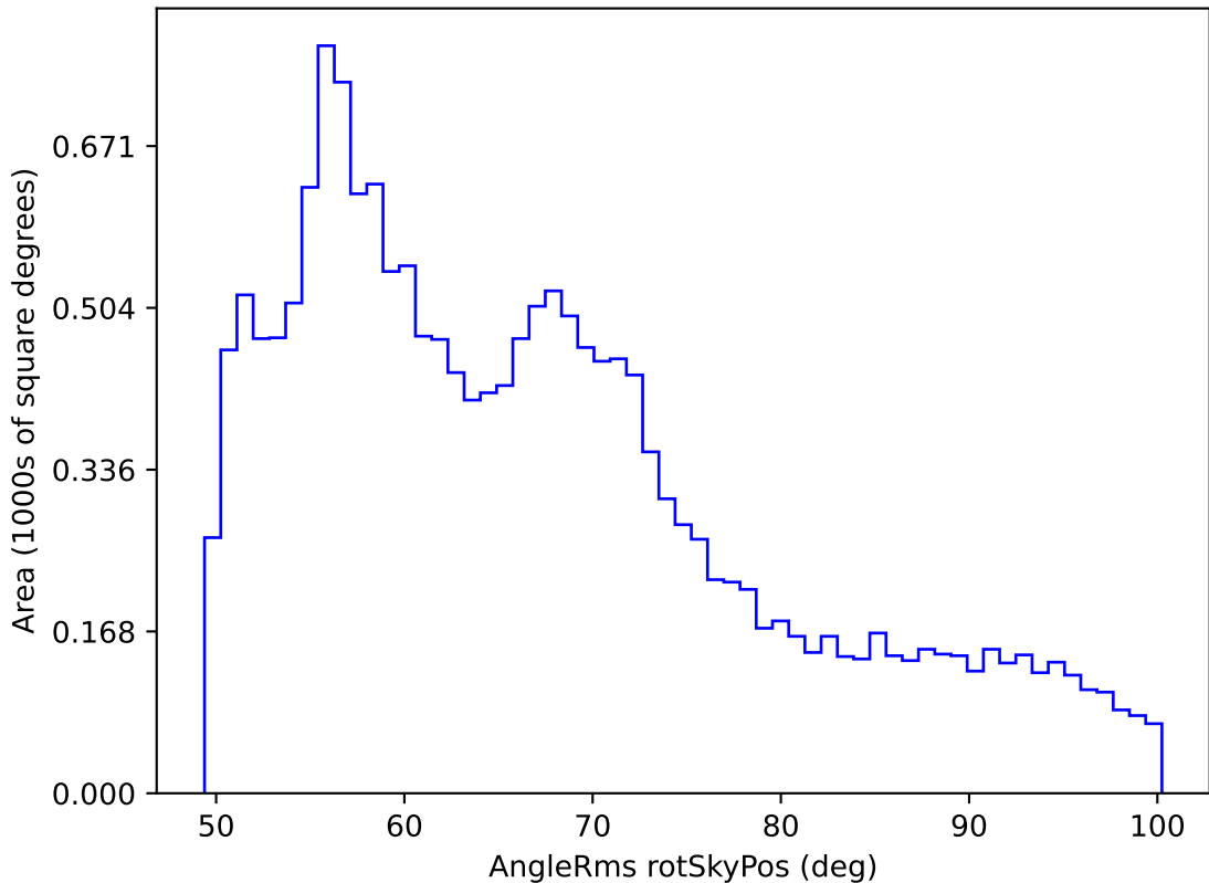
weather_cloudso31v3.4_10yrs WFD all bands: AngleRms rotSkyPos
