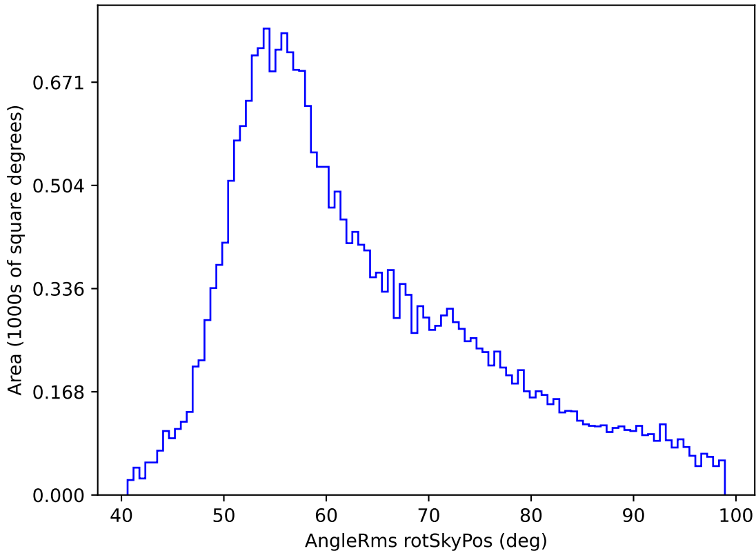
weather_cloudso31v3.4_10yrs All sky z band: AngleRms rotSkyPos
