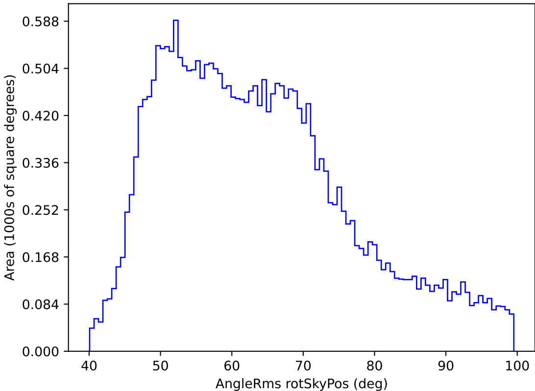
weather_cloudso31v3.4_10yrs All sky r band: AngleRms rotSkyPos
