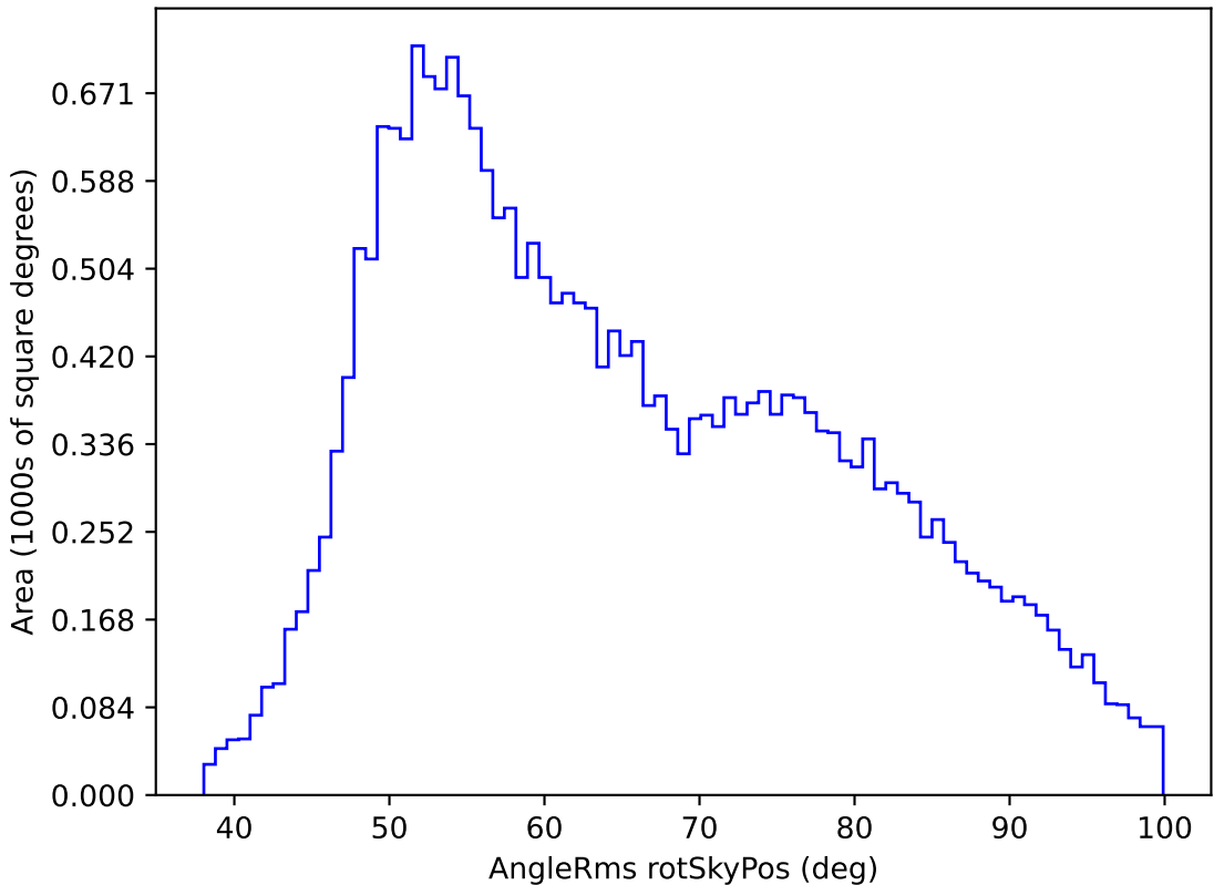
weather_cloudso31v3.4_10yrs All sky g band: AngleRms rotSkyPos
